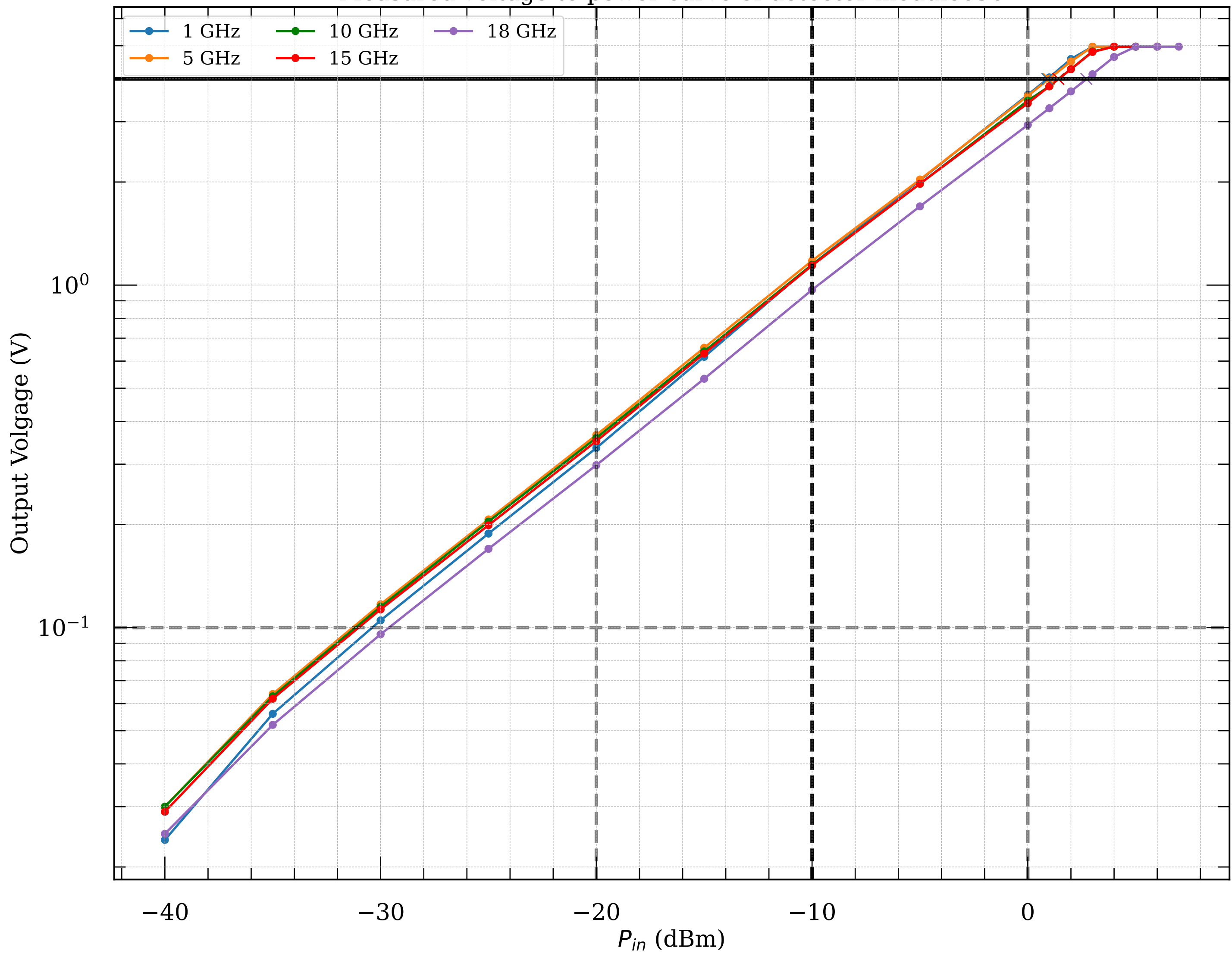
Measured voltage-to-power curve of detector module090
